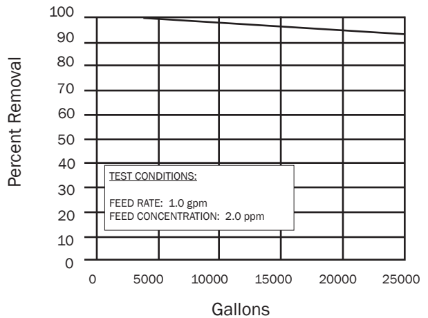
S7010-14 Hydro-Cure® GAC/KDF Cartridge Typical Chlorine Removal Rate
